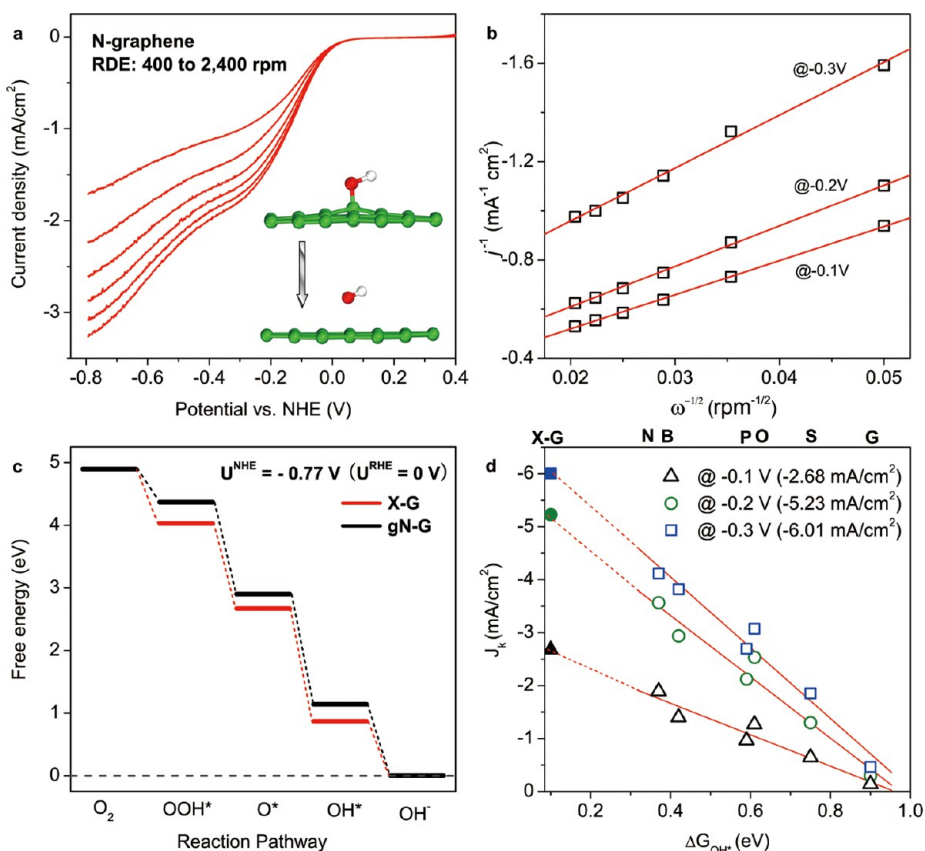
Figure 7. (a) Electrochemically measured LSV of N-graphene catalyst at different rotating speeds in an O_2 -saturated 0.1 M solution of KOH. Inset illustrates the last electron transfer step: OH^* desorption to generate OH^- . (b) Koutecky–Levich plots for N-graphene at -0.3 V, -0.2 V, and -0.1 V vs NHE, data were collected from panel a. (c) Potential corrected free energy diagram for gN-G and X-graphene models at U^{RHE} = 0 V ( U^{NHE} = -0.77 V). (d) The relationship between \Delta G_{OH^*} and j_k for various synthesized graphene catalysts under different potentials (open symbols), data were collected from Figure S3, SI. The values in parentheses of the legend are j_k values for X-graphene, which are predicted by extending the fitted lines to \Delta G_{OH^*} = 0.10 eV, shown as closed symbols.
